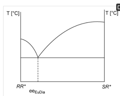
Figure 2. Binary melting phase diagram of a diastereomeric mixture of RR^* and SR^* [3,6] and the possibility of calculating the achievable F value using the ee_{Dia} (Equation (2)).
