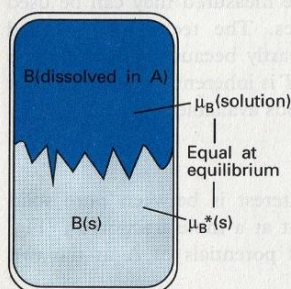
7.17 The heterogeneous equilibrium involved in the calculation of the solubility is between pure solid B and B in the mixture.
