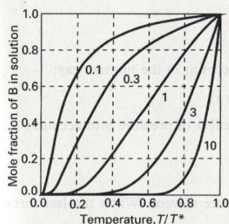
7.18 The variation of solubility (the mole fraction of solute B in a saturated solution) with temperature ( T^* is the freezing temperature of the solute). Individual curves are labelled with the value of \Delta_{fus}H/RT^* .
